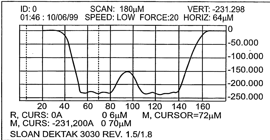
SURFACE TOPOGRAPHY SCANS FOR THE ANNULI OF FIG. 10
